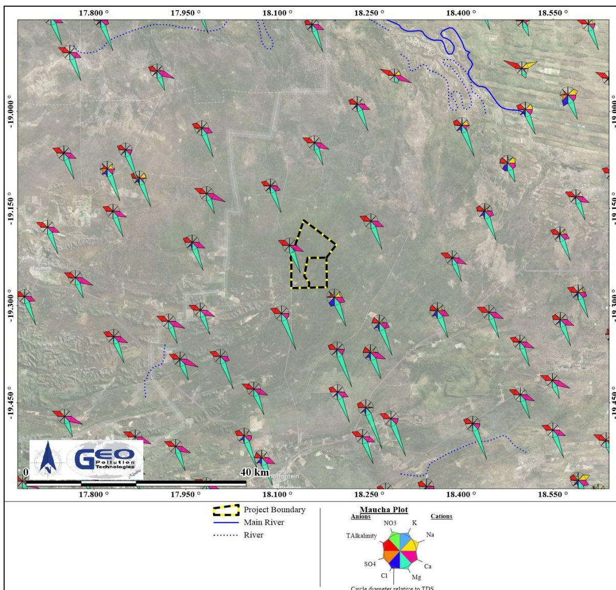
Figure 7-8 Groundwater quality
