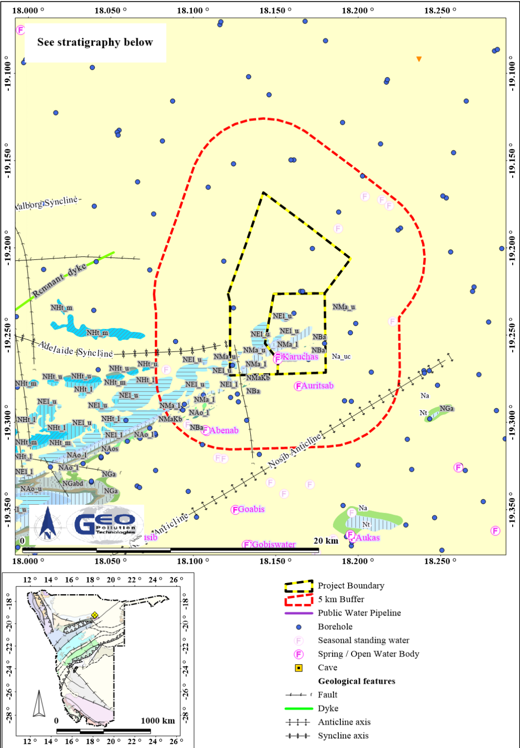
Figure 5-5 Hydrogeological map
