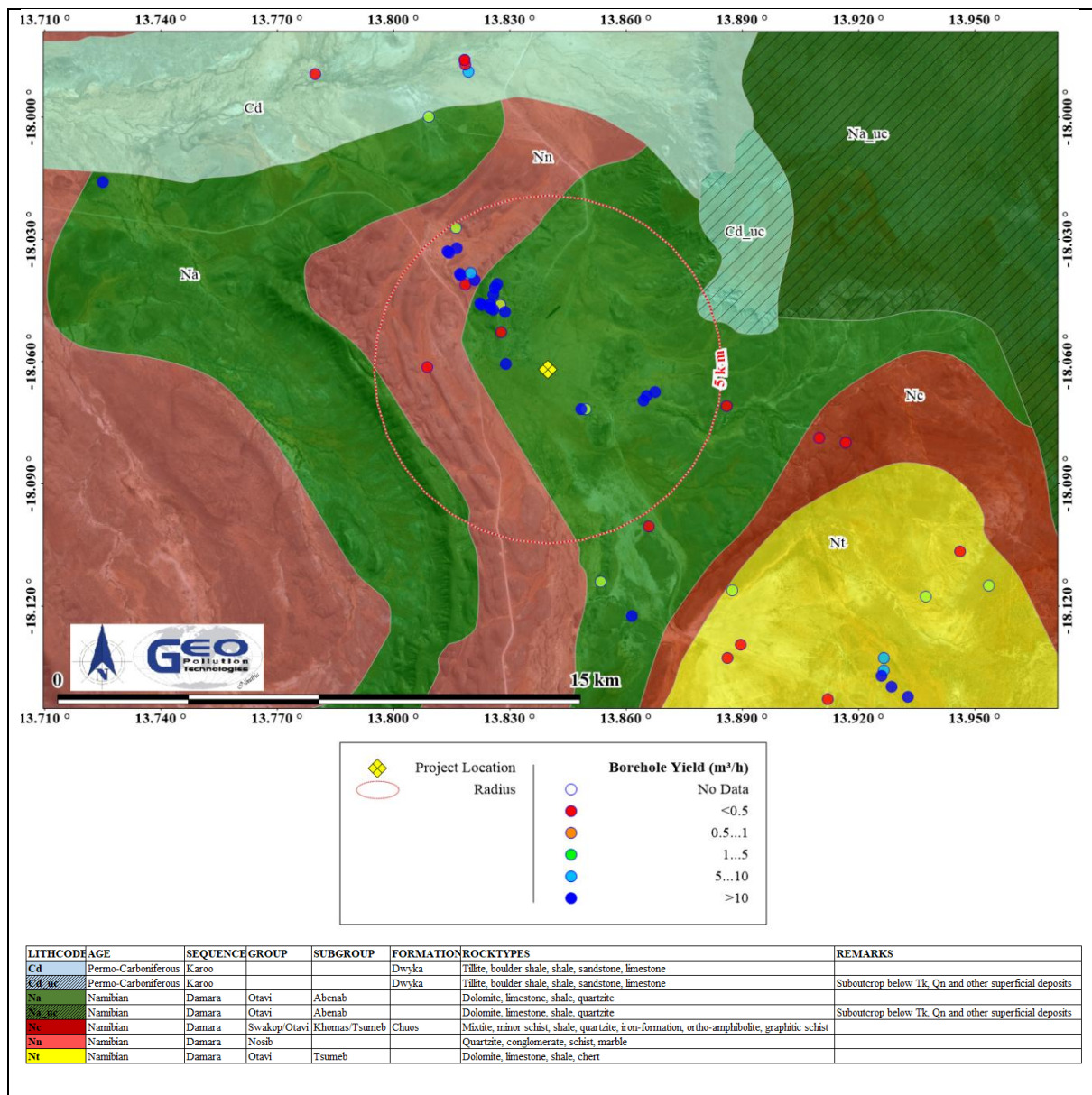
Figure 7-5. Geology Map
