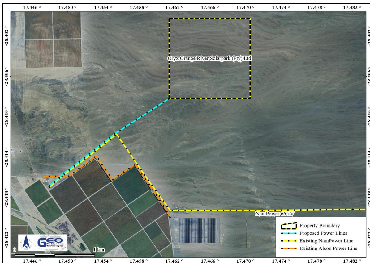
Figure 5-2 Proposed location of the site and related power line
