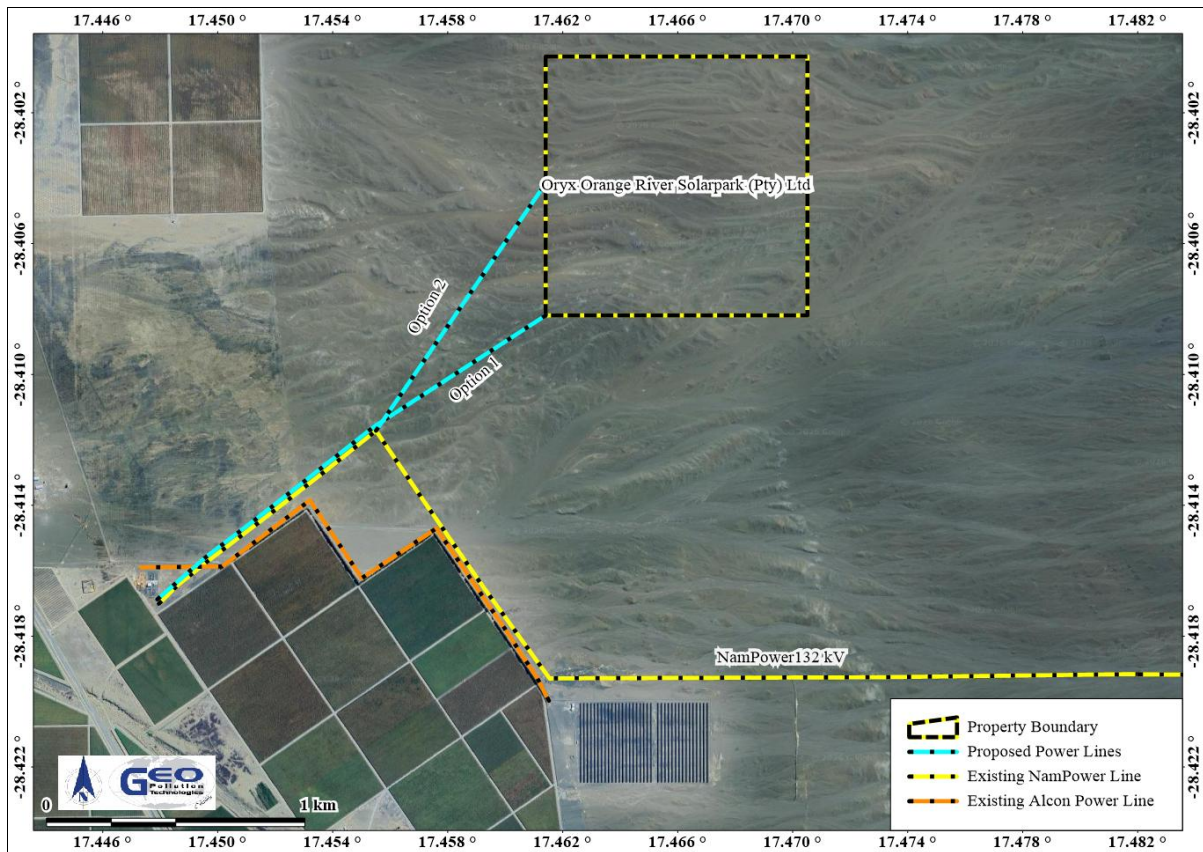
Figure 6-3 Alternative power line options
