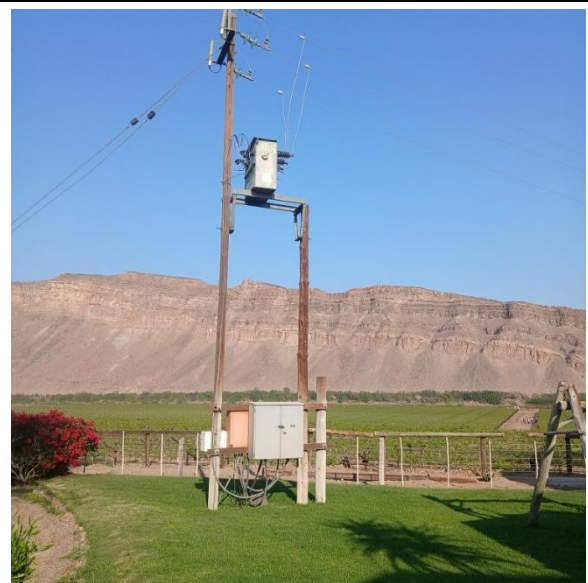
Photo 3-8 NamPower transformer
