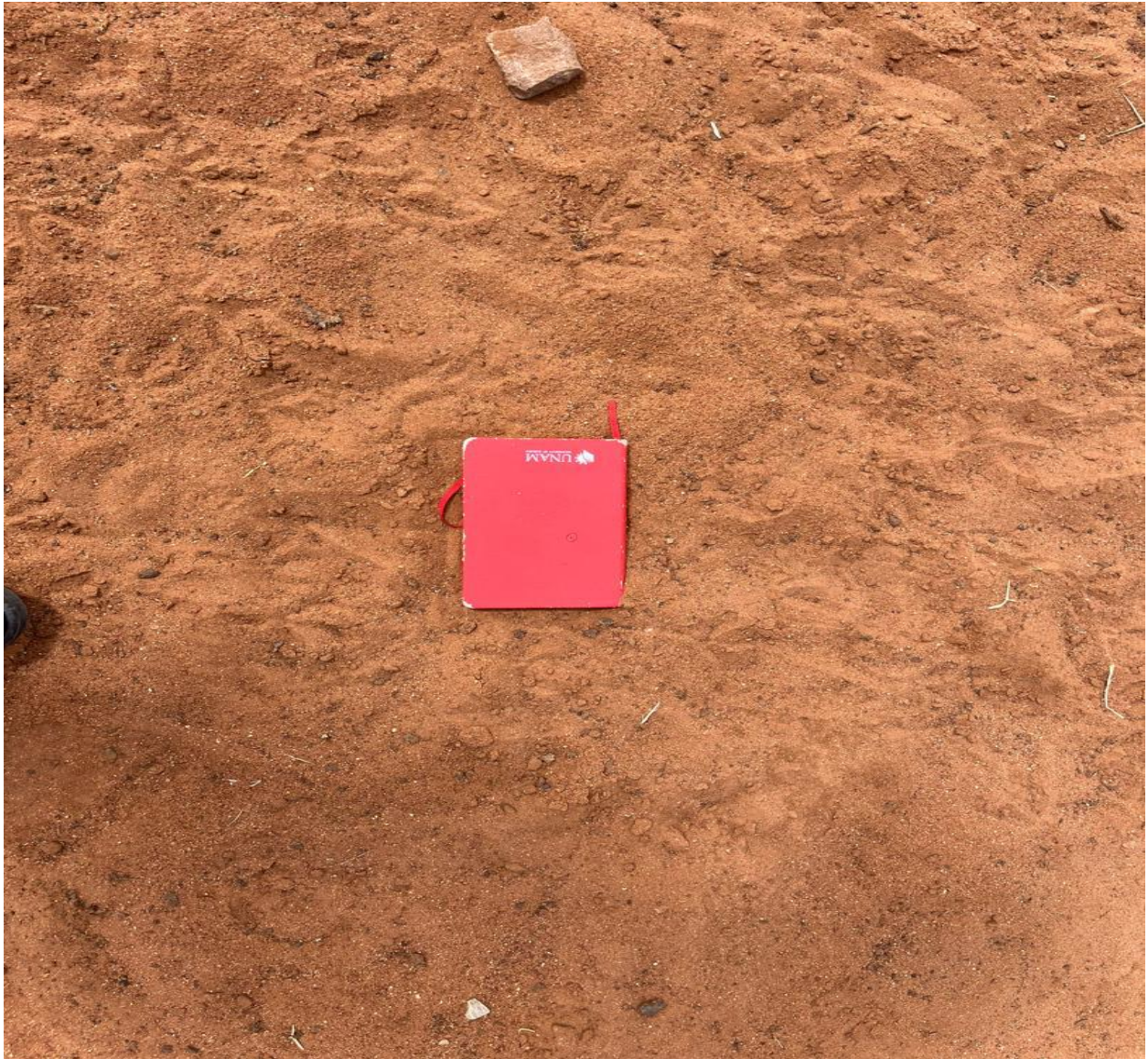
Figure 8: Reddish, sandy Chromic Cambisol observed in EPL 10774 area.
