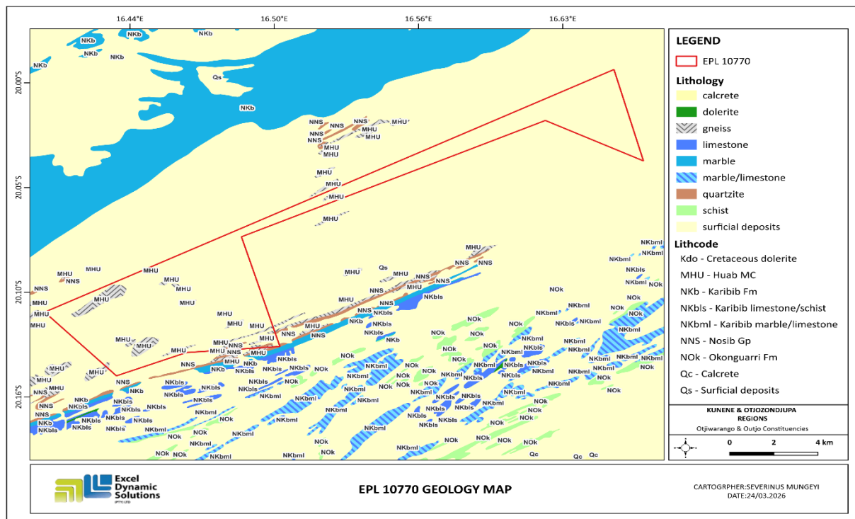
Figure 5: Geological map of the project area
