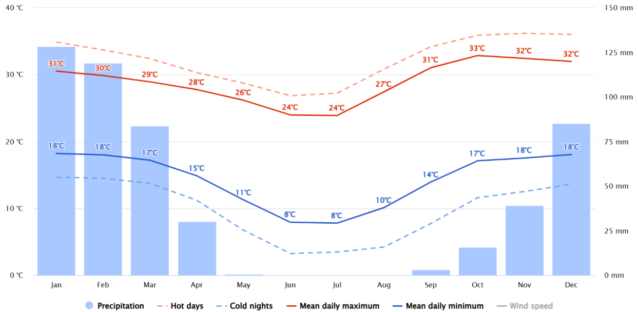
Figure 3: Climatic patterns of the project area
