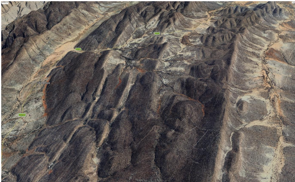
Figure 5. The topographical geomorphology for the mining claims area.
