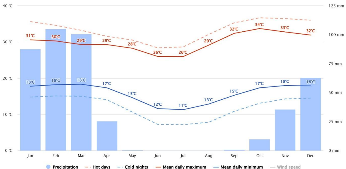
Figure 4. The long term climatic condition for the mining claims area.
