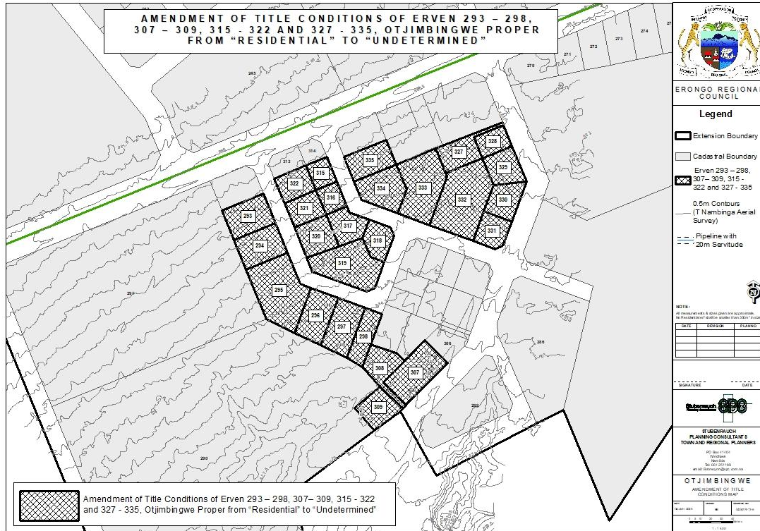
Figure 6: Amendment of Title Conditions of Erven 293 – 298, 306 – 309, 315 - 322 and 327 - 335, Otjimbingwe Proper from “Residential” to “Undetermined”
