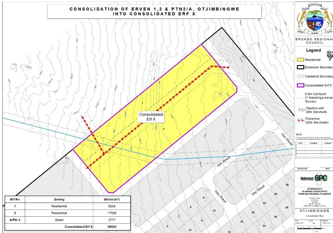
Figure 5: Consolidation of Erven 1 and 2, & PTN/A, Otjimbingwe into “Consolidated Erf X”
