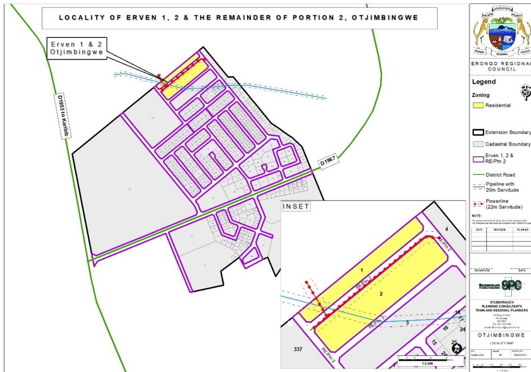
Figure 1: Locality of Erven 1, 2 & the Remainder of Portion 2, Otjimbingwe
