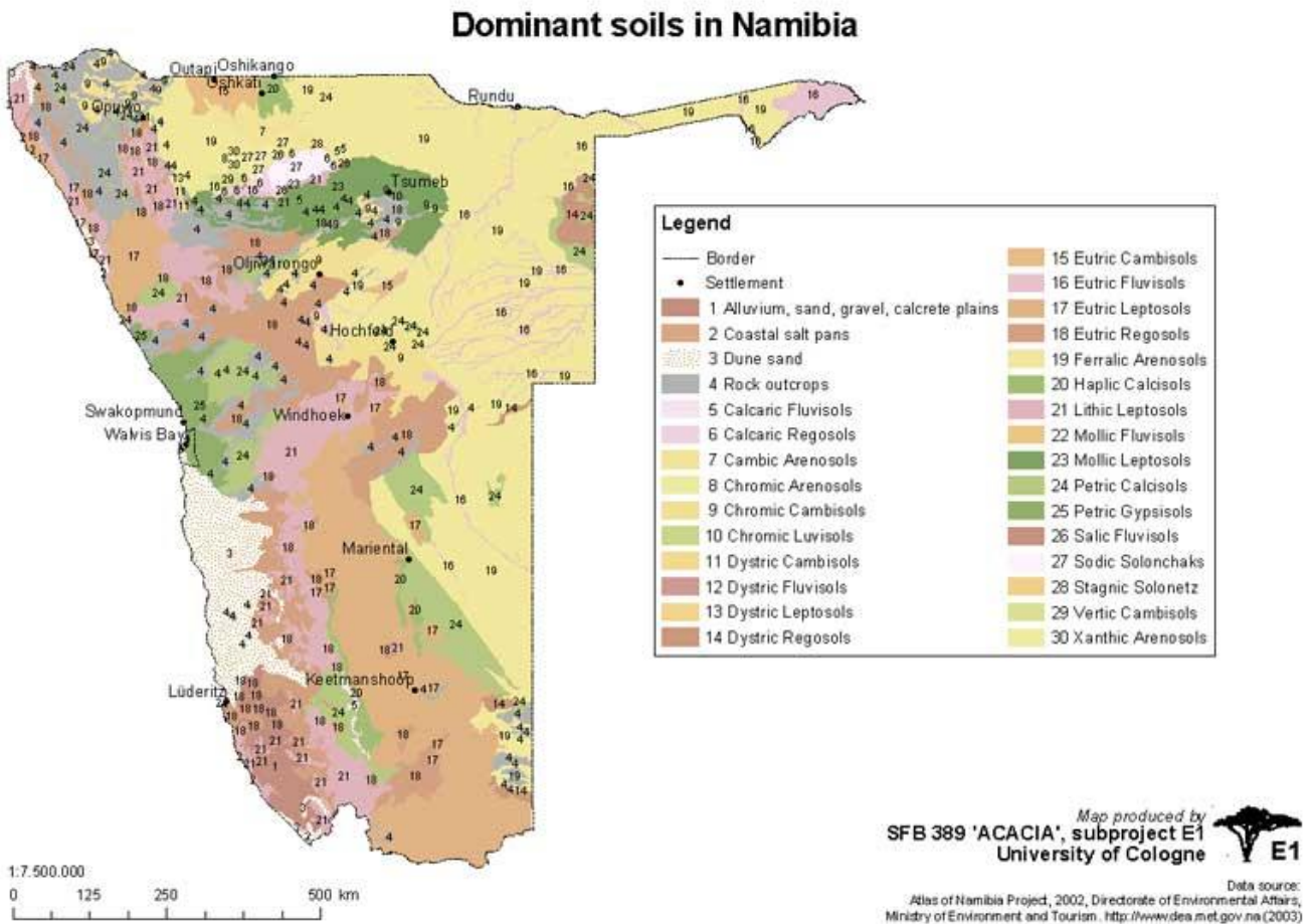
Figure 3-11: Dominant Soils in Namibia
