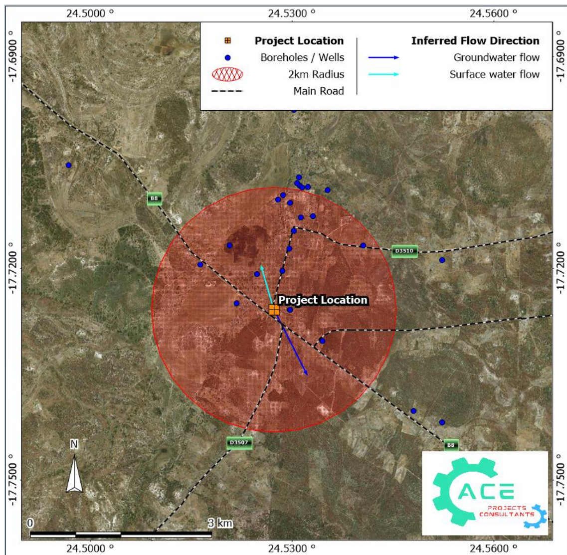
Figure 2. Hydrogeological Map
