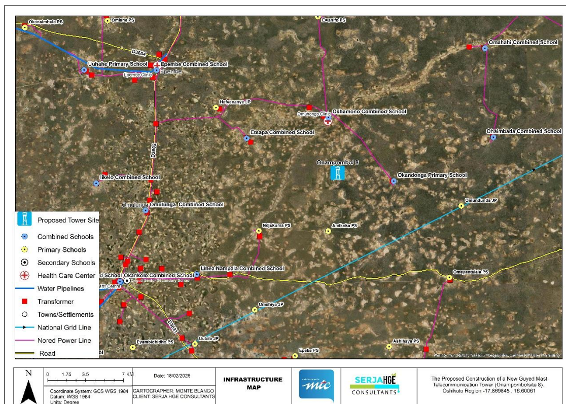
Figure 5-7: The infrastructure map of the Onampombo Village and surrounding areas
