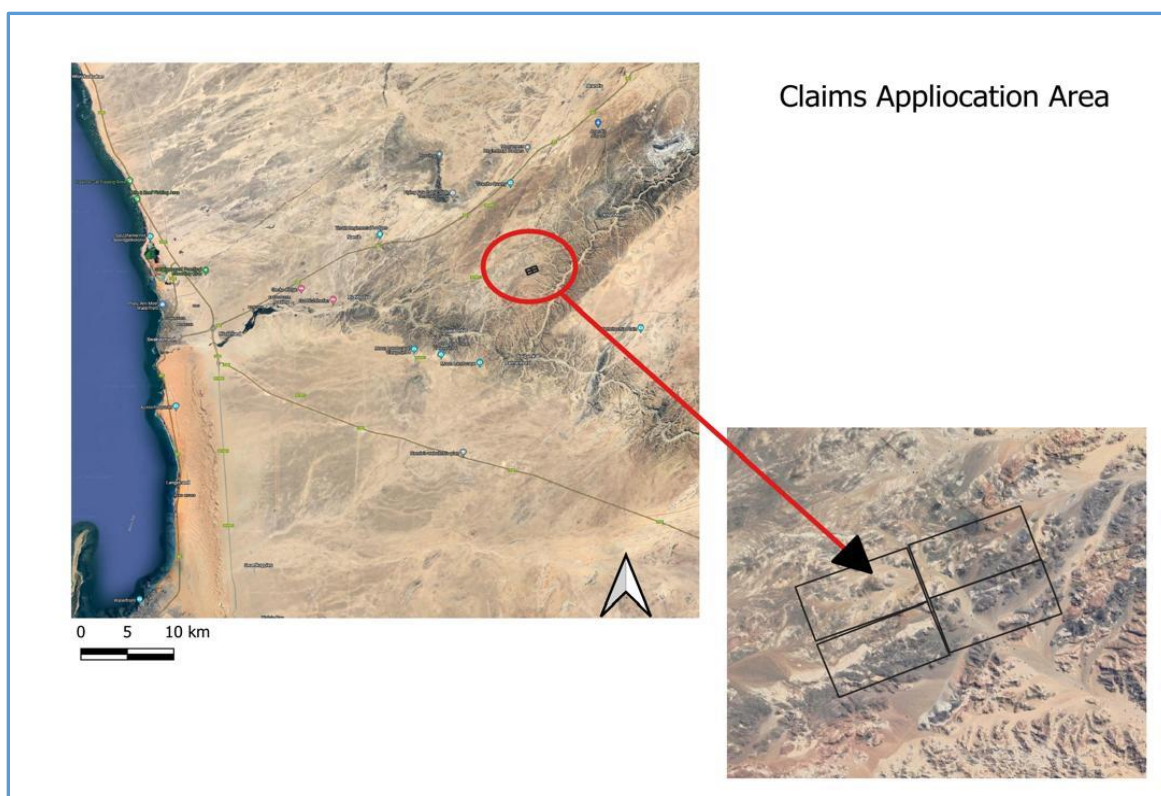
Figure 1: Geological locality map of the proposed mining activities (CL 75286, 75287, 75288 and 75251).
