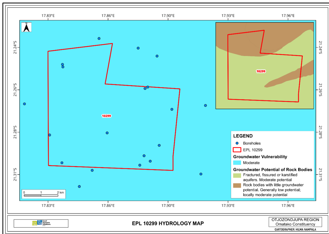
Figure 8: Hydrology map for EPL 10299
