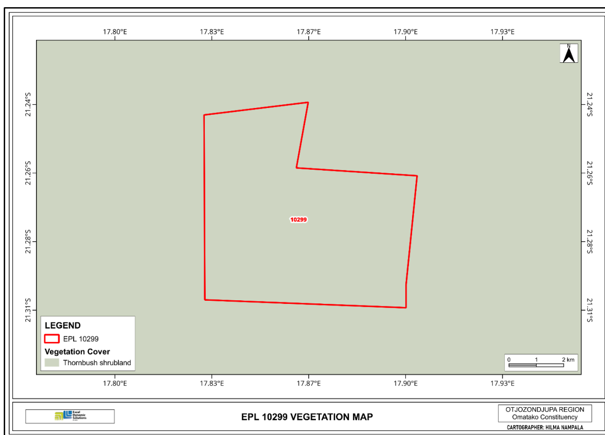
Figure 9: Vegetation map - EPL 10299
