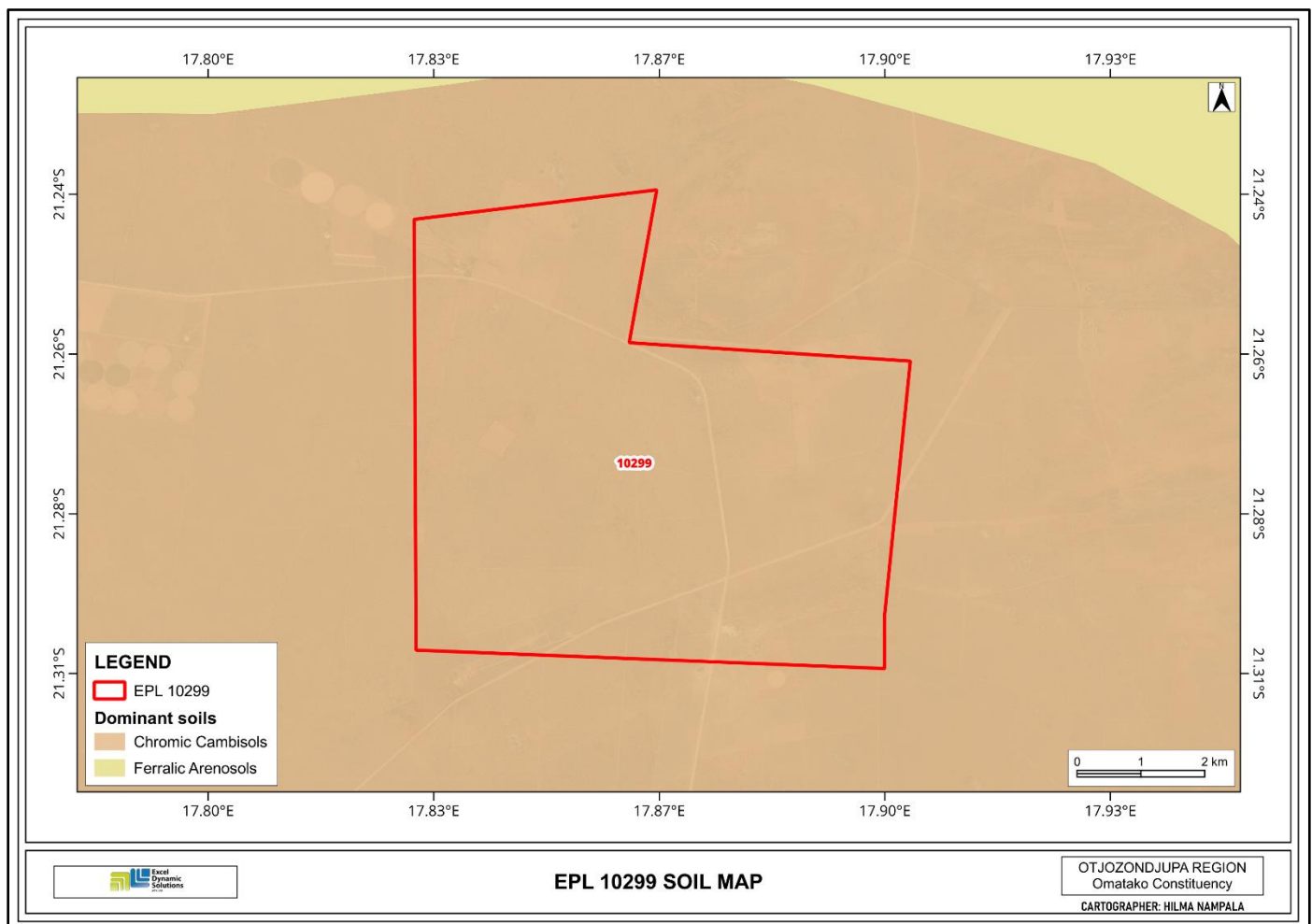
Figure 6: Soils map for EPL 10299
