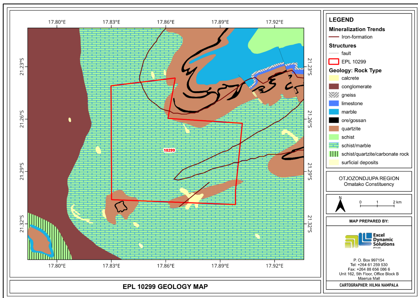
Figure 5: General Geology map for EPL 10299
