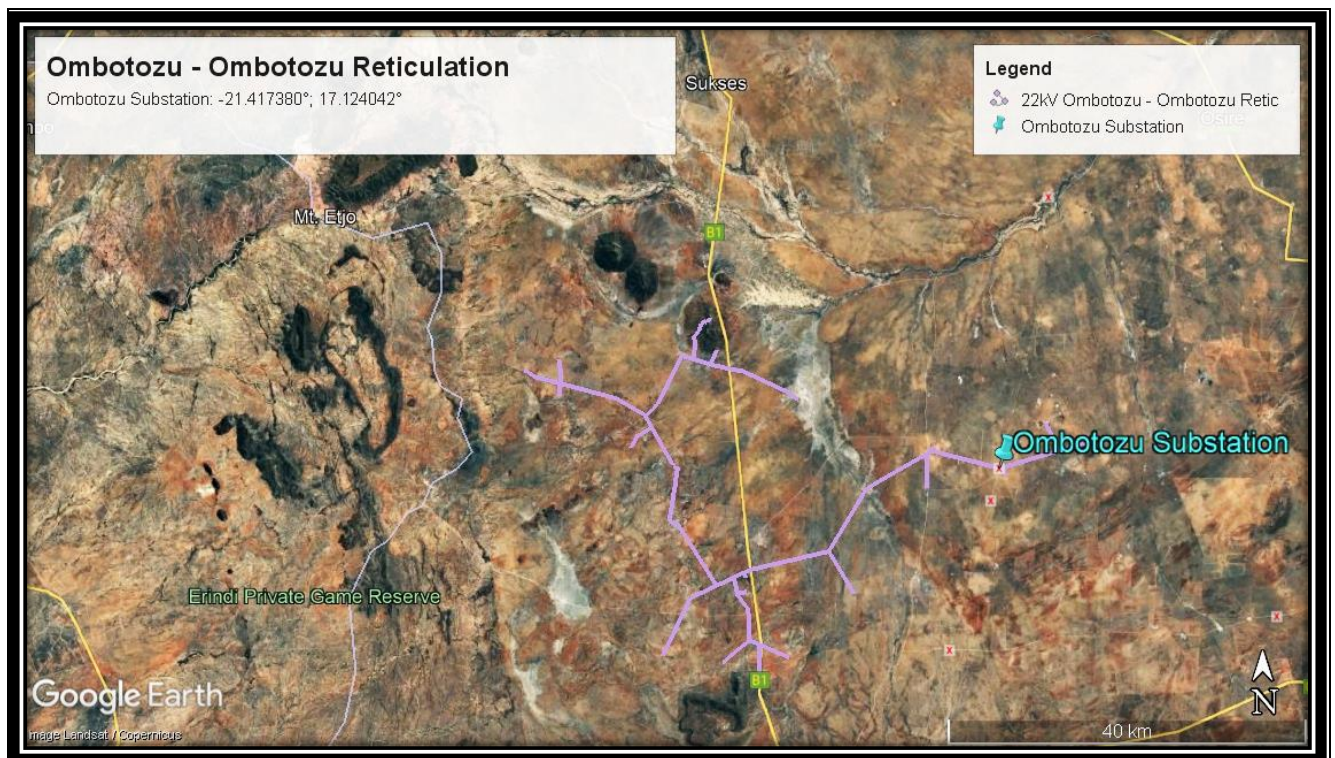
Figure 1: Locality map showing the Ombotozu - Ombotozu reticulation system
