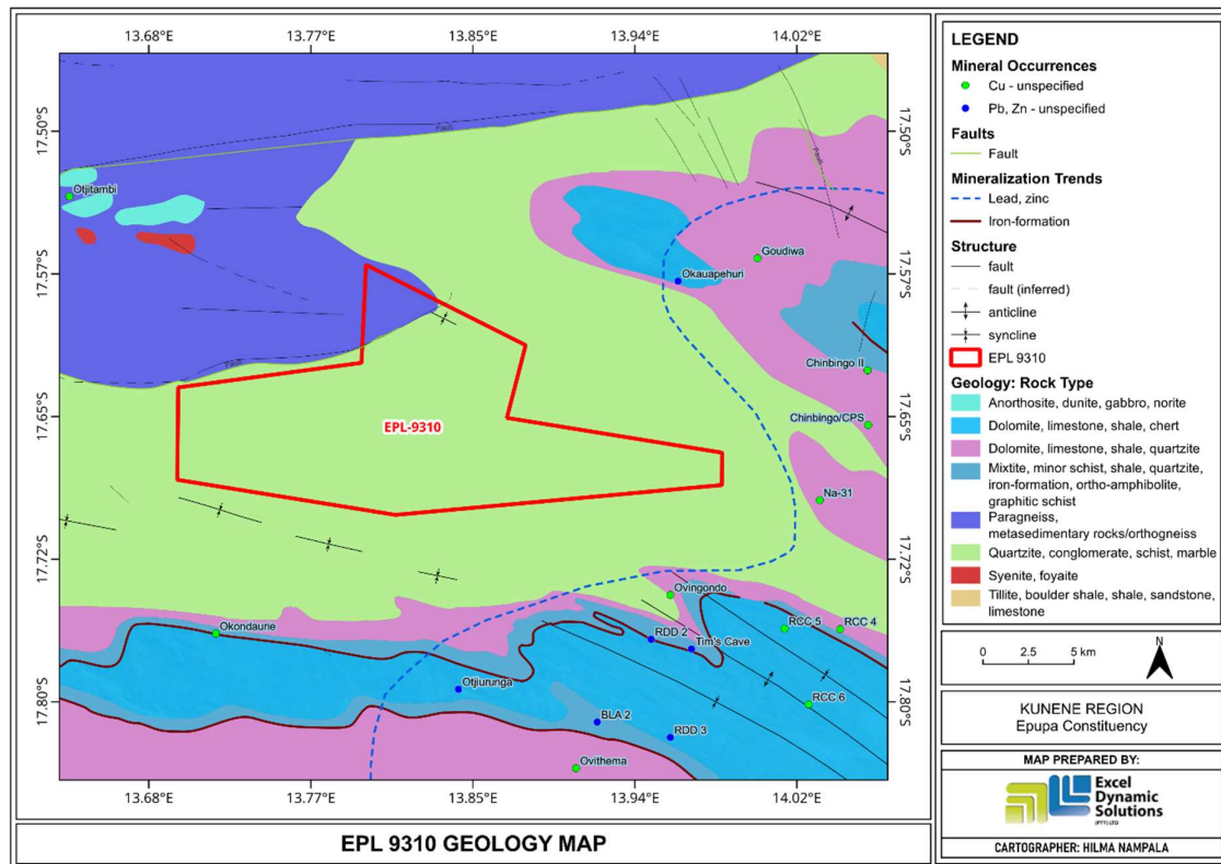
Figure 6: Geology map – EPL 9310.
