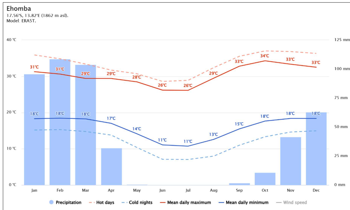
Figure 3: Climate Conditions in Ehomba (source: (Meteoblue, N.D))
