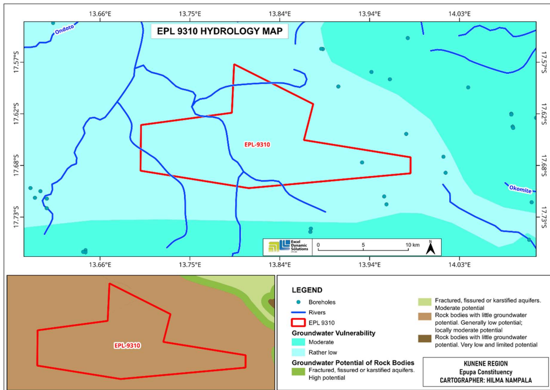
Figure 9: Hydrological map on EPL 9310.
