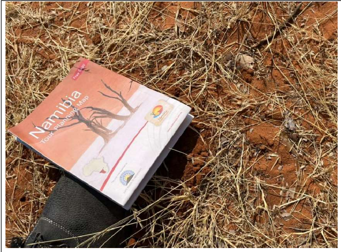
Figure 8: Type of soil observed on the EPL.
