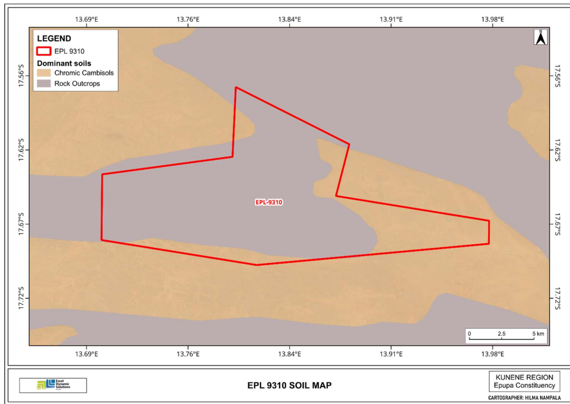
Figure 7: Soil Map for EPL 9310.
