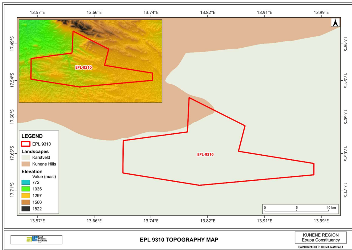
Figure 4: Topography Map for EPL 9310.
