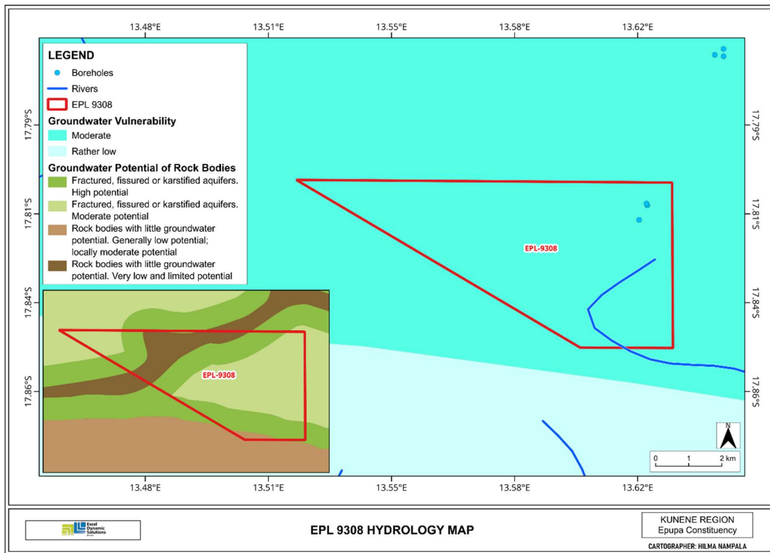
Figure 9: Hydrological map on EPL 9308.
