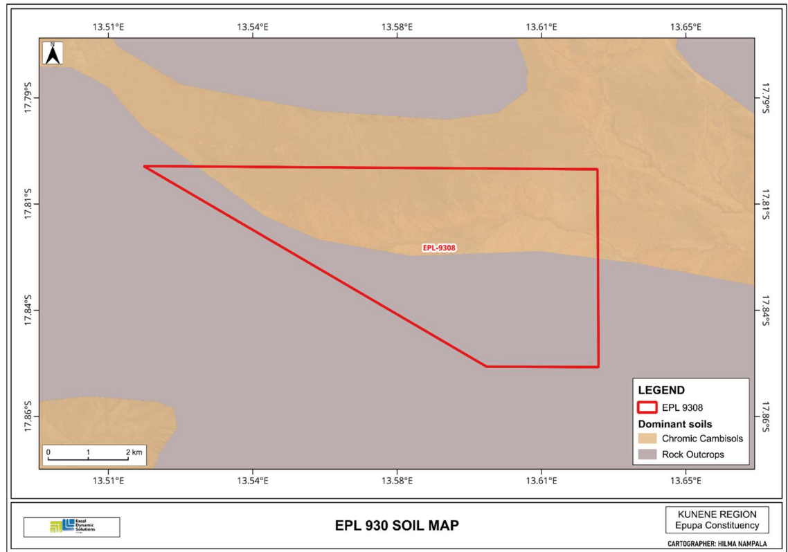
Figure 7: Soil Map for EPL 9308.
