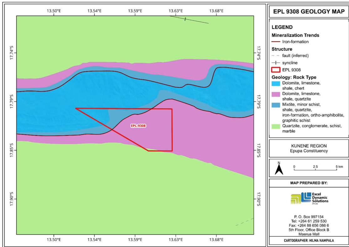
Figure 6: Geology map – EPL 9308.
