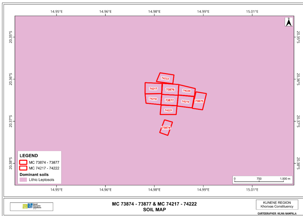
Figure 6: Dominant soil type on the MCs
