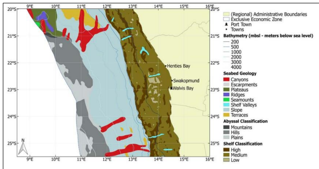
Figure 16: Seafloor geomorphic features. Source: MFMR 2018
