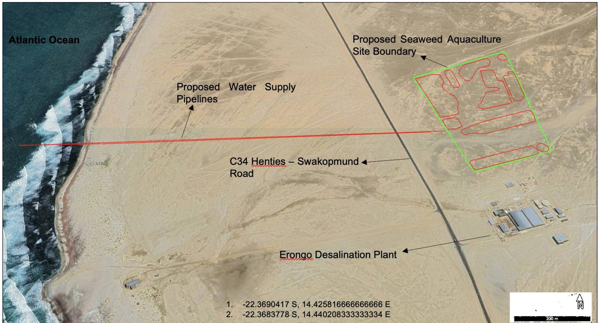
Figure 2: Proposed Pipeline Route
