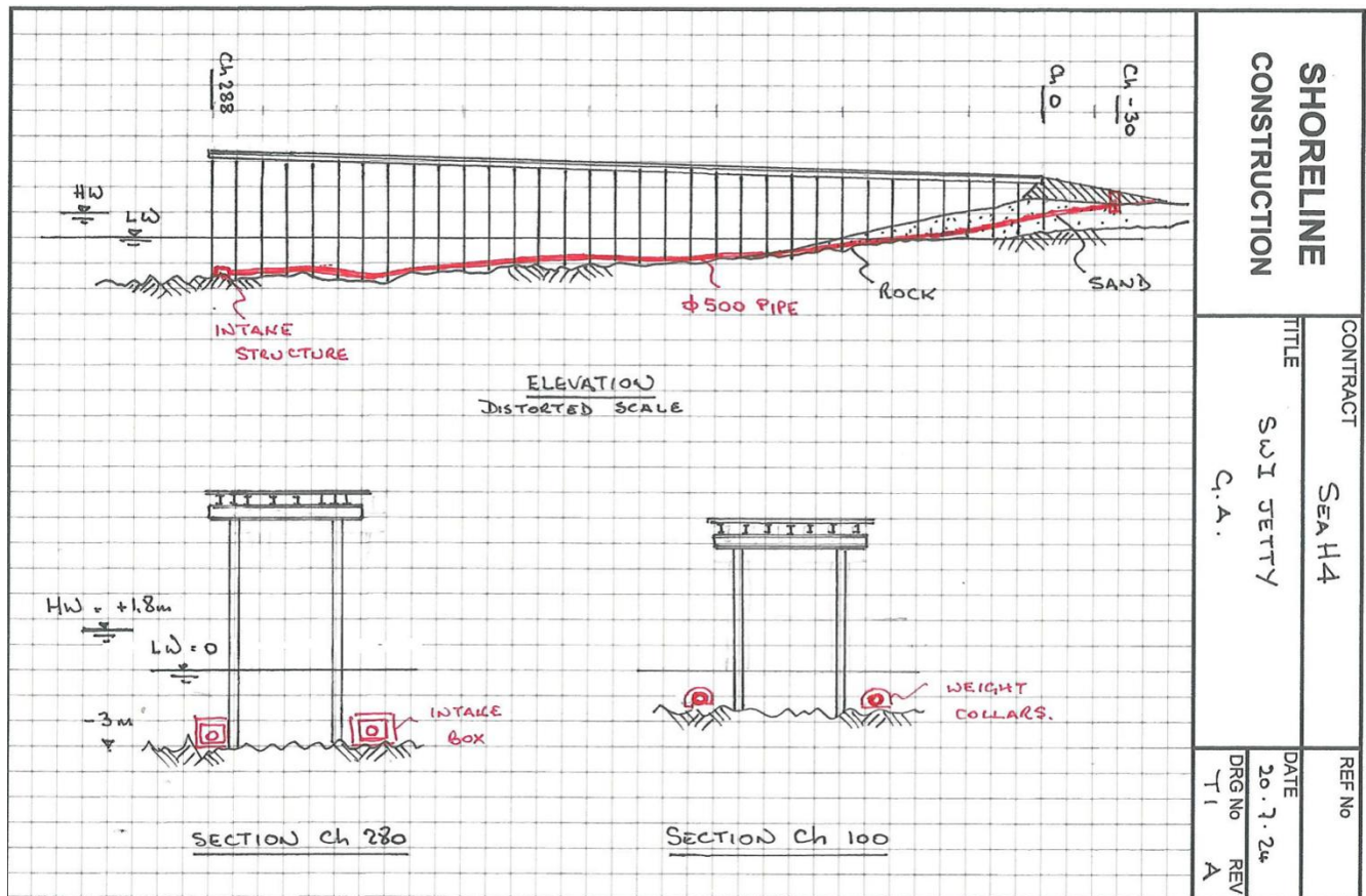
Figure 9: Steel Jetty Design
