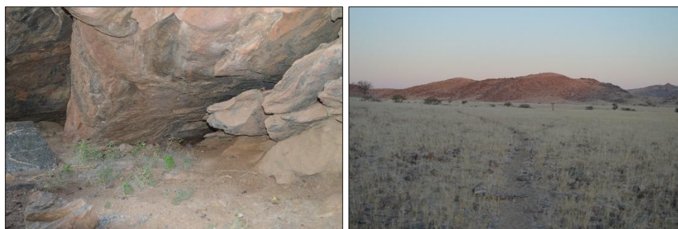
Figure 5-8: Photos of the rock units in the visited areas of the EPL
