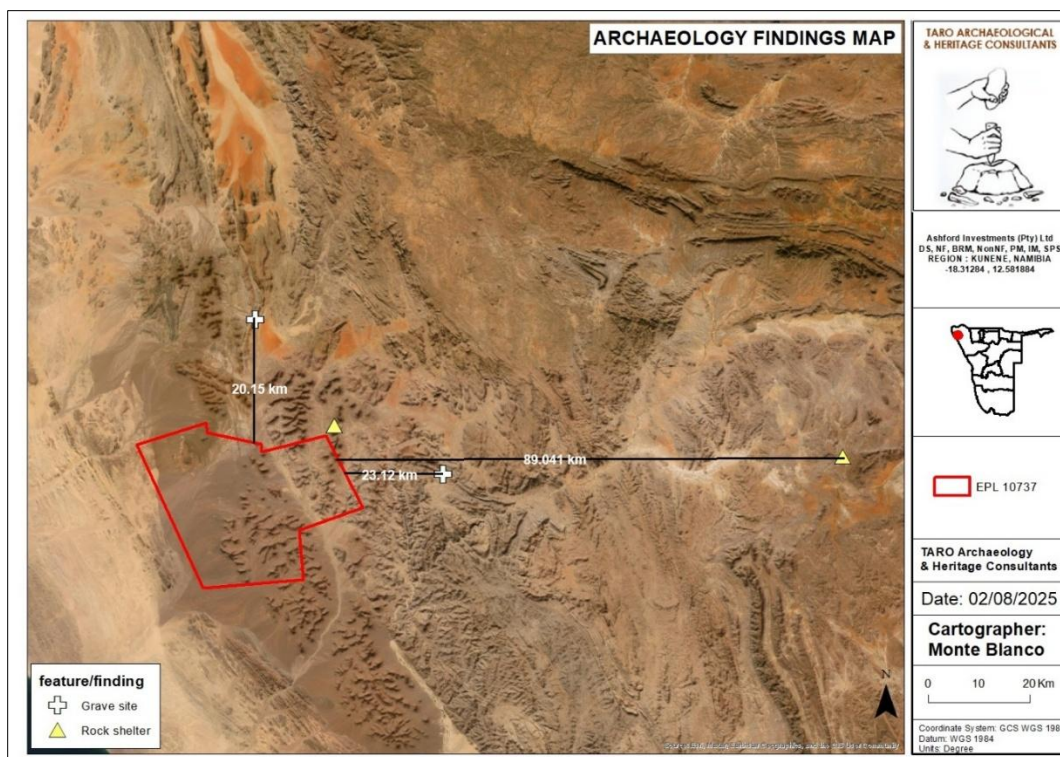
Figure 5-16: Archaeological findings map (Mushi, 2025)
