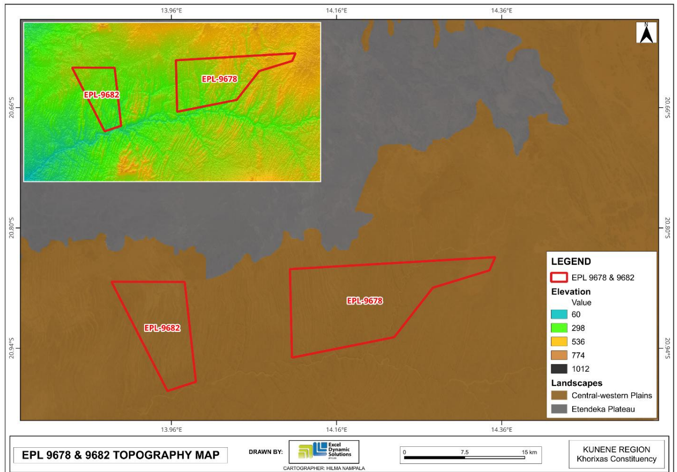
Figure 3: The Topography and landscape map for the project area.
