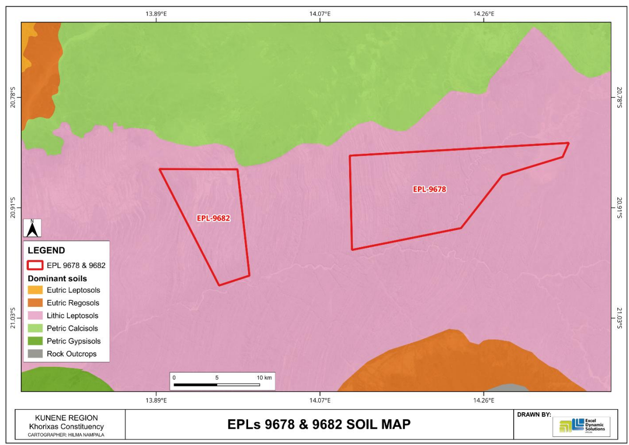
Figure 8: Soils map for EPL 9682 and 9678
