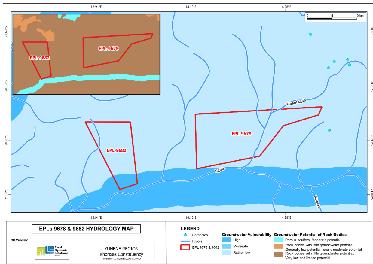
Figure 10: Hydrology map for EPL 9682 and 9678.
