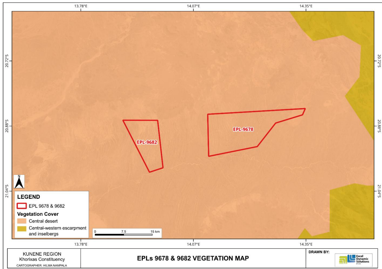
Figure 12: Vegetation map - EPL 9678 and 9682.
