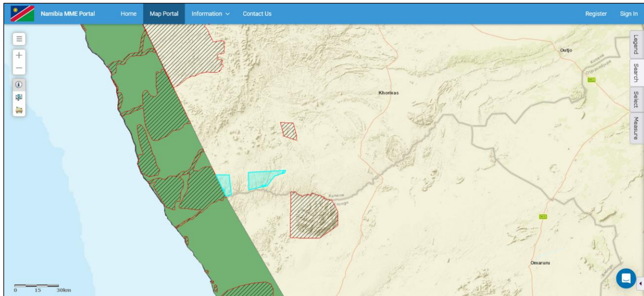
Figure 2: Location of EPL 9678 and 9682 (National Mining Cadastre ( https://maps.landfolio.com/Namibia/ ))
