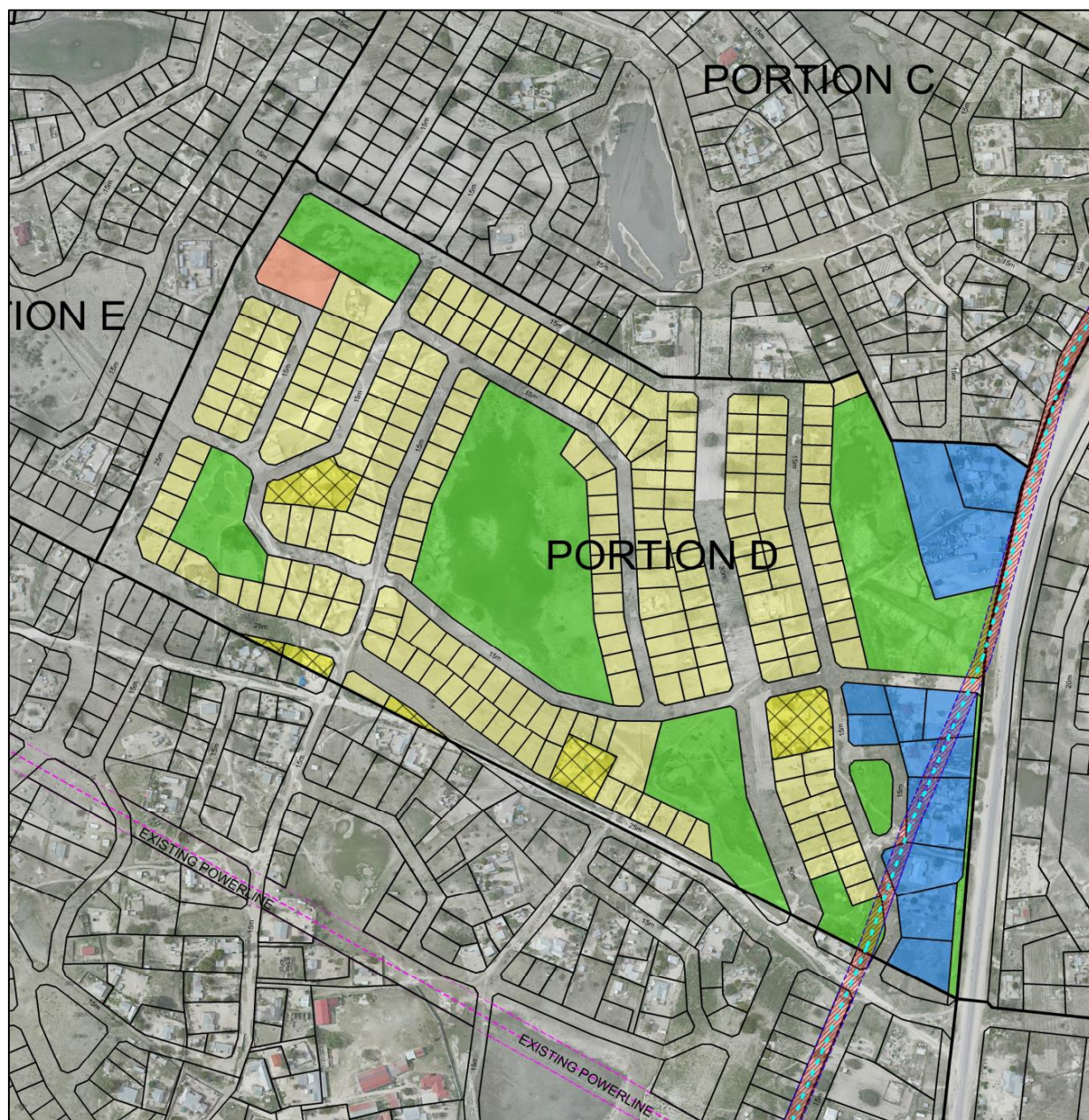
Proposed layout on Portion D
