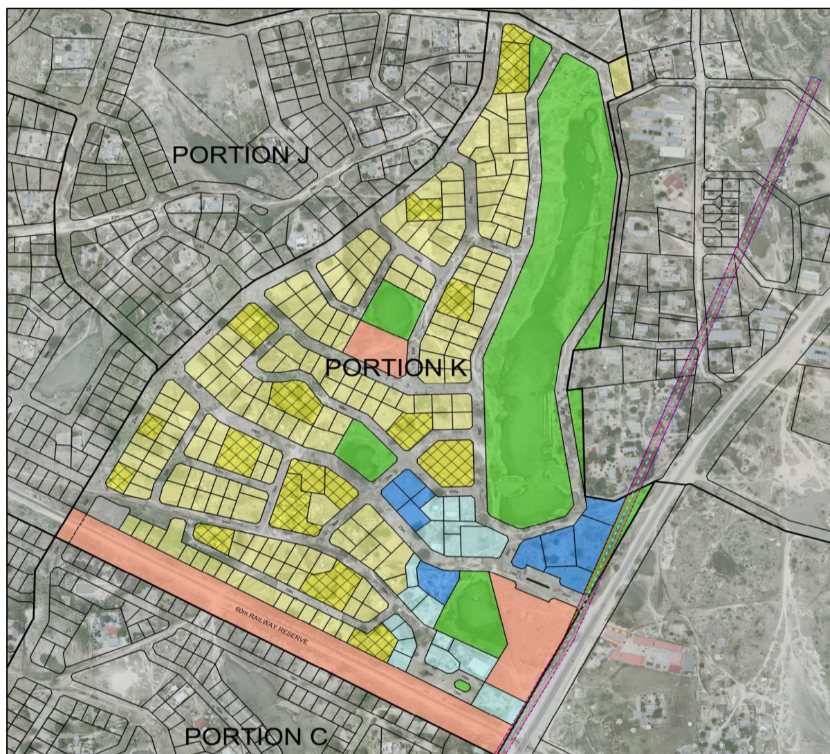
Proposed layout on Portion K
