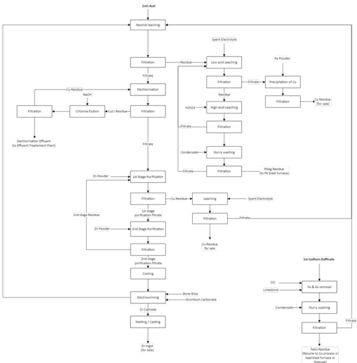
Figure 3.6: Zinc Oxide Hydrometallurgical treatment block flow diagram
