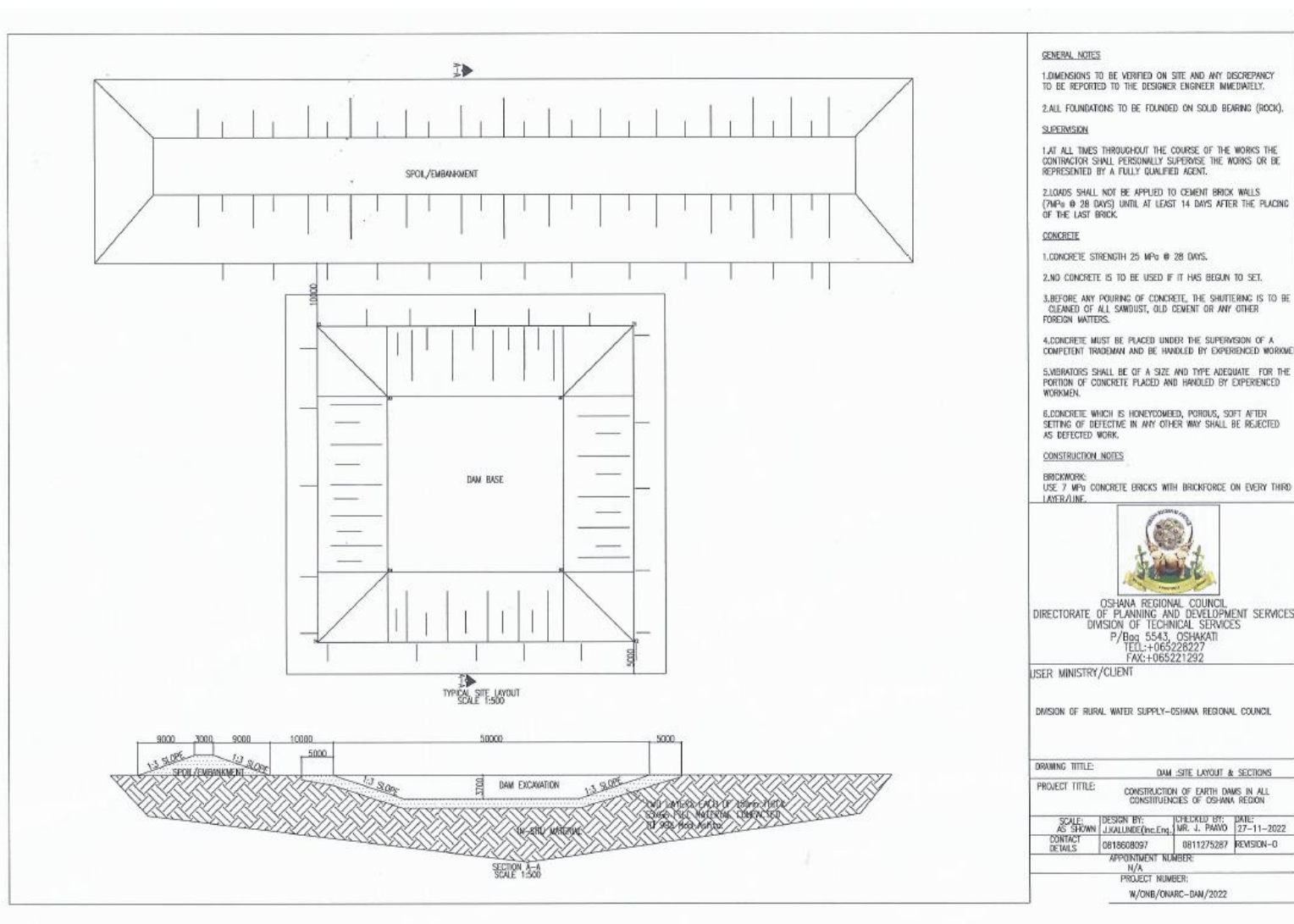
Figure 2-5: Earth Dam Design
